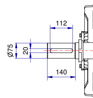
Shaft detail
