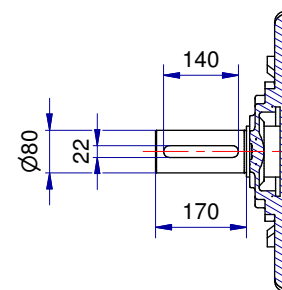
Shaft detail
