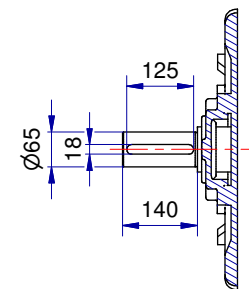
Shaft detail
